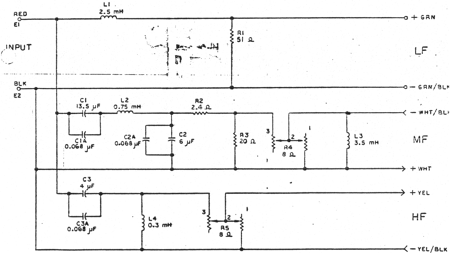
SIMPLIFIED SCHEMATIC
